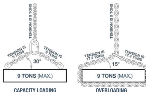
FIGURE 2 5/8" CM Herc-Alloy 800® ALLOY STEEL CHAIN SLINGS
