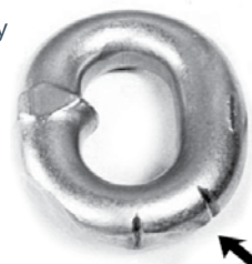
Figure 2: Location of nicks, gouges, and notches will dictate their severity.
