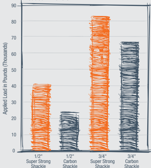
The Comparative Strength of the Shackles Loaded in Tension
