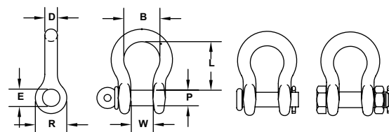
Screw Pin
