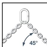
DOUBLE, DOUBLE ENDLESS* OR SINGLE BASKET
