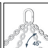
TRIPLE, QUADRUPLE OR DOUBLE BASKET
